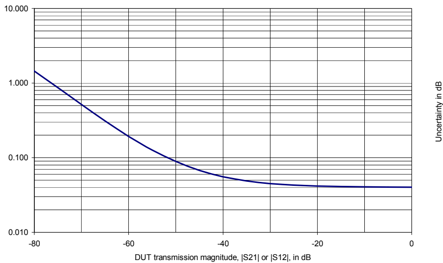
Transmission magnitude uncertainty with calibration method "Full Two Port High Accuracy", f = 1 GHz, IF bandwidth = 100 Hz.
