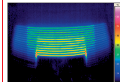
Fault in heating of rear window
