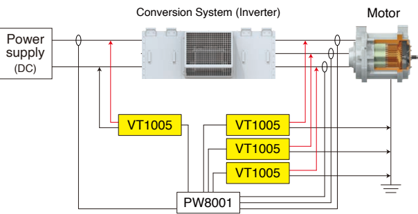
Evaluation of the Efficiency of Inverters that use SiC Power Devices in Electrical Railways Example of VT1005 and PW8001 connection
