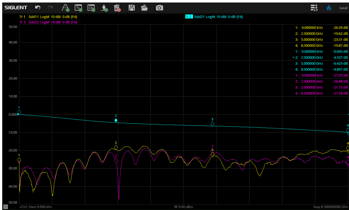
Figure 4-17 Test result of differential line
