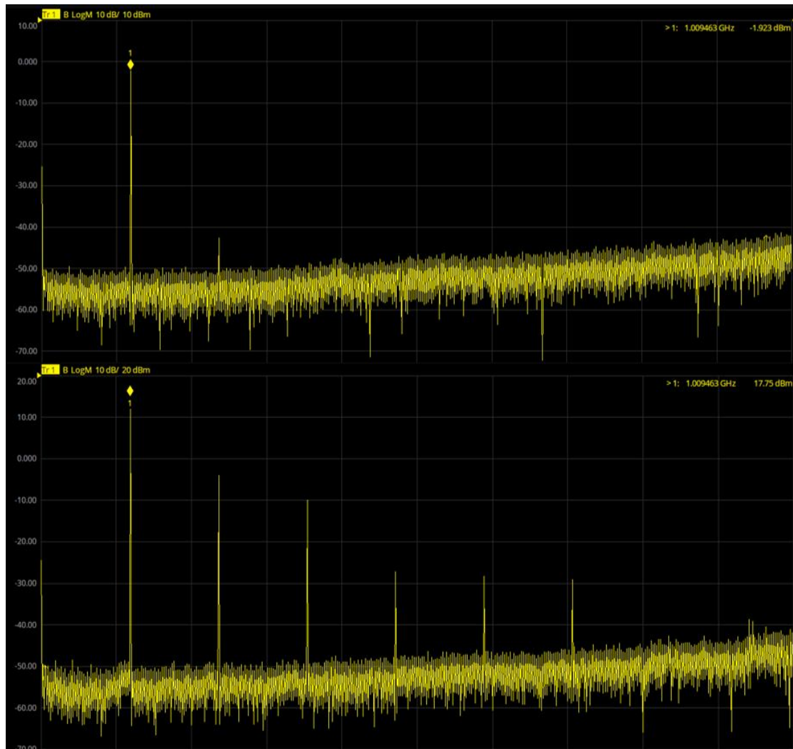
Figure 4-6 Spectrum test result of the linear (upper) and nonlinear (lower) regions of the amplifier
