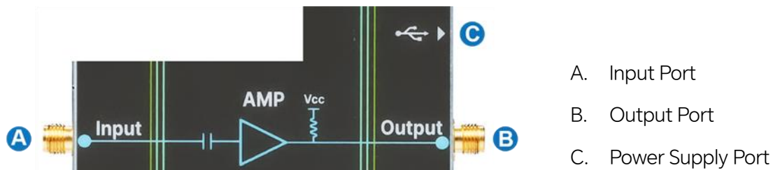
Figure 3-4 Schematic diagram of amplifier module
