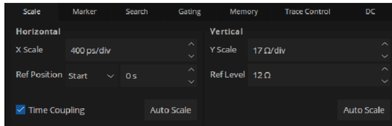
Figure 4-14 TDR axes scale adjustment
