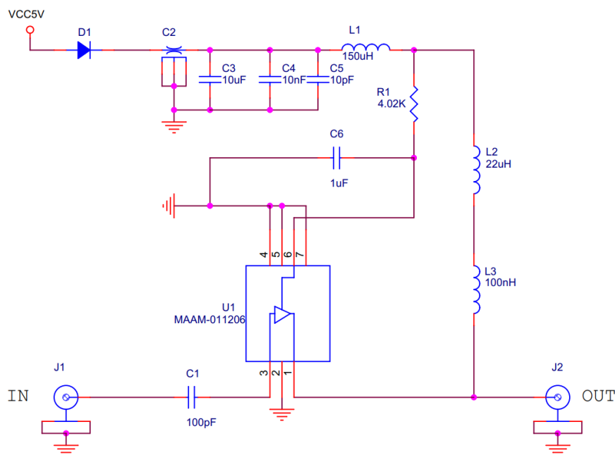
Figure 3-5 Schematic diagram of amplifier module
