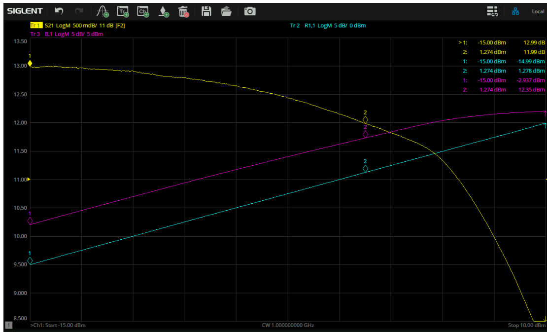
Figure 4-4 Test result of amplifier with power sweep
