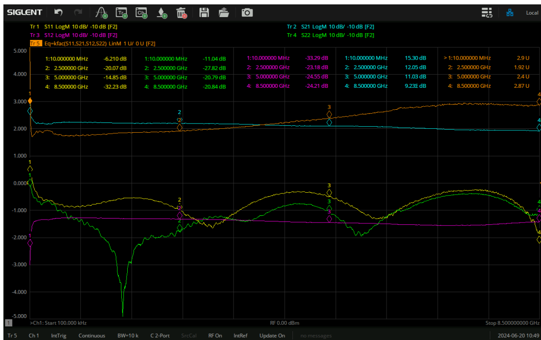
Figure 4-3 Test result of amplifier with linear frequency sweep
