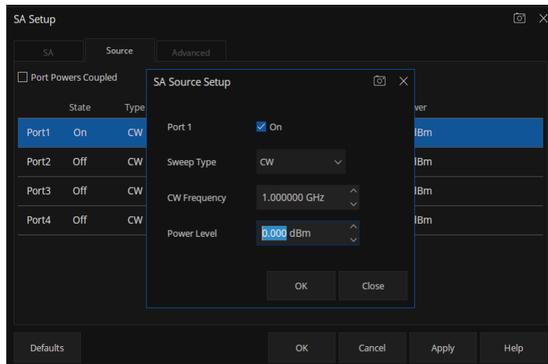
Figure 4-5 SA Source Setup interface for amplifier input port
