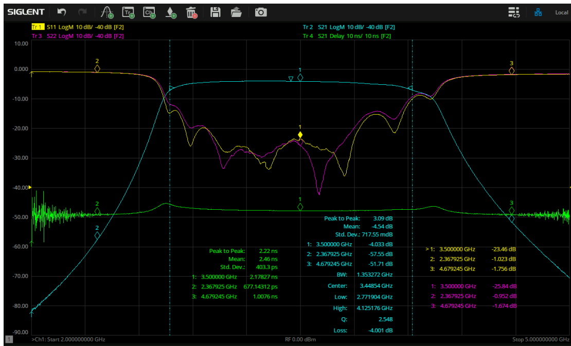
Figure 4-9 Test result of band-pass filter
