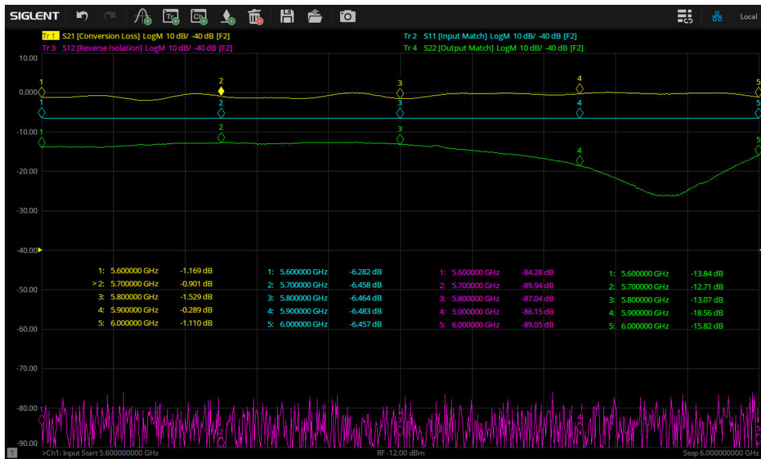
Figure 4-2 Test result of mixer
