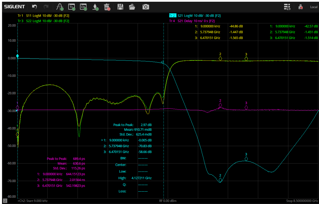
Figure 4-10 Test result of low-pass filter
