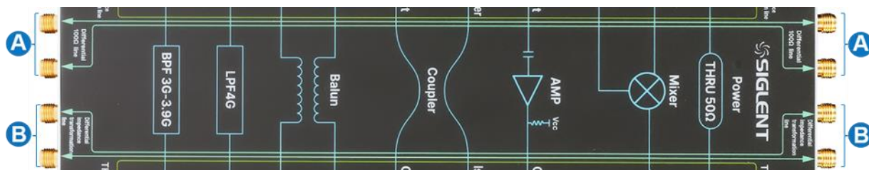
Figure 3-10 Schematic diagram of differential line and differential impedance transformation line
