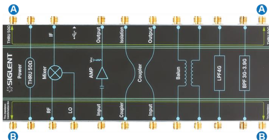
Figure 3-9 Schematic diagram of long through line and impedance transformation line
