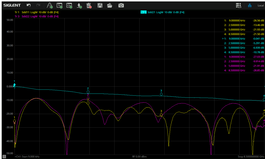
Figure 4-18 Test result of differential impedance transformation line
