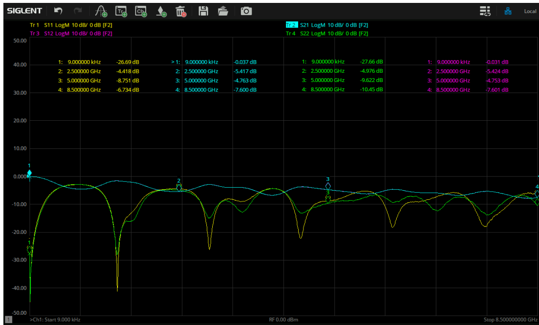
Figure 4-13 Test result of impedance transformation line
