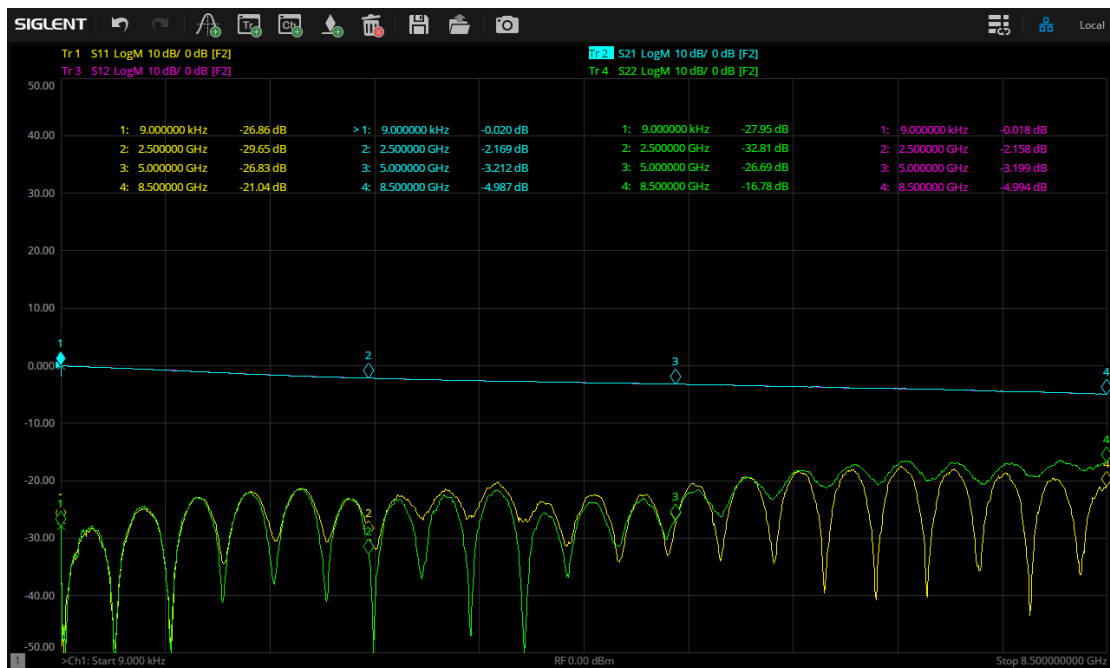
Figure 4-12 Test result of long through line
