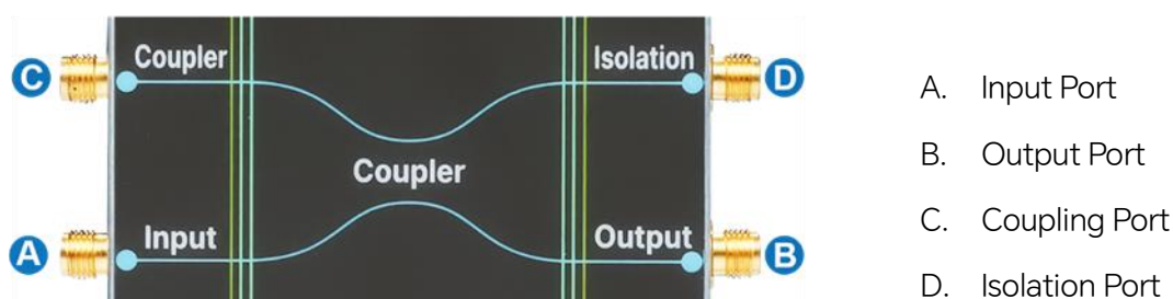
Figure 3-6 Schematic diagram of coupler
