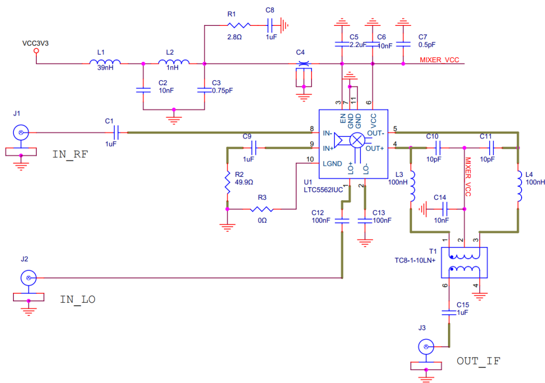
Figure 3-3 Mixer module schematic diagram
