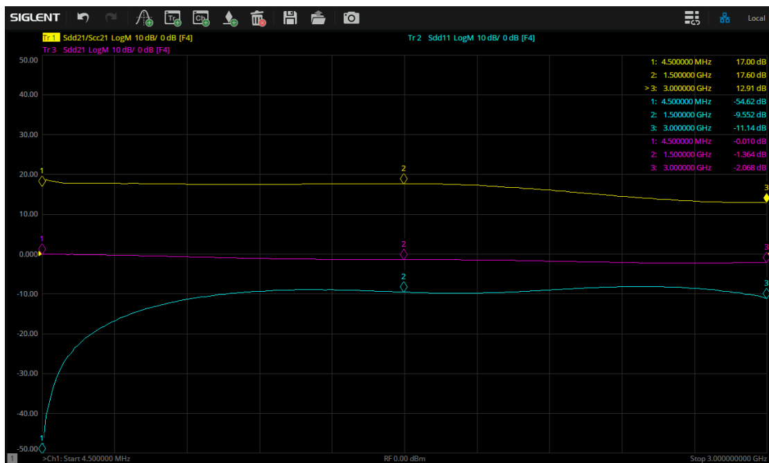
Figure 4-8 Test result of balun
