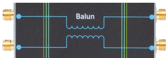
Figure 3-7 Schematic diagram of balun
