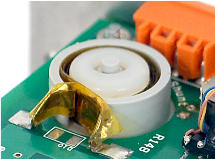
Spiral Shunt for 1 A input
