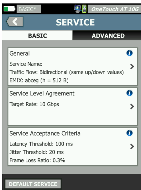
Figure 17: 10G NPT test threshold for frame loss rate, jitter and latency using up to 9300 bytes user defined frame size.
