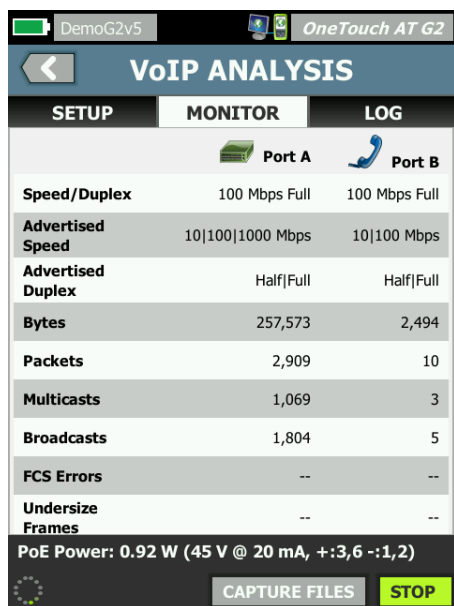
Figure 27: Inline VoIP analysis simplifies troubleshooting of desktop VoIP problems in real-time without TAPS or switch mirror ports.
