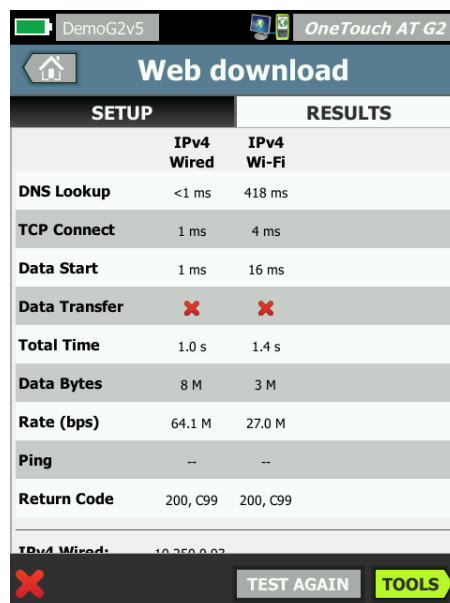
Figure 9: Detailed breakdown of network-hosted application performance including return code of web transaction. This level of detail allows quick isolation of issues when tests fail.
