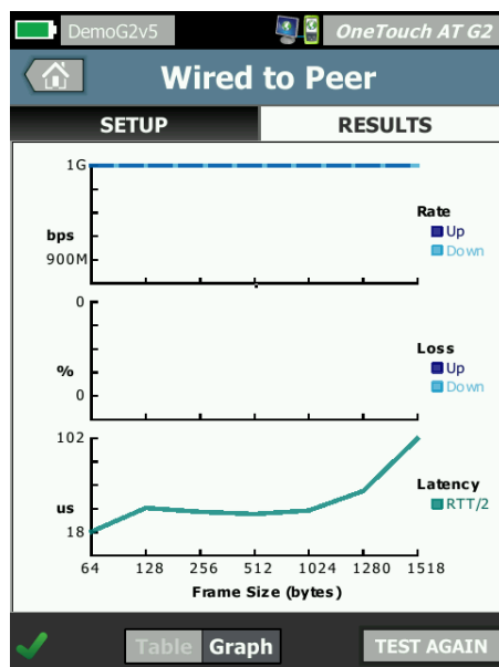
Figure 12: End-to-end path performance measurement validates link readiness and SLA compliance.
