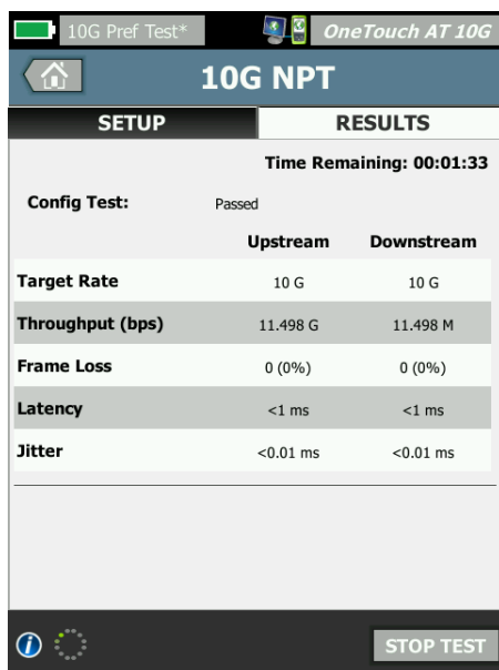
Figure 19: Detailed test results of upstream and downstream against a peer.
