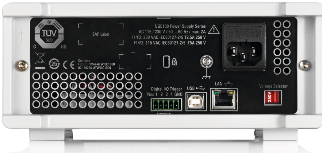
Rear view of the R&S®NG100 series.
