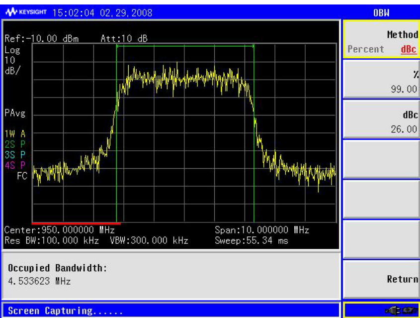
The occupied bandwidth measured in dBc.
