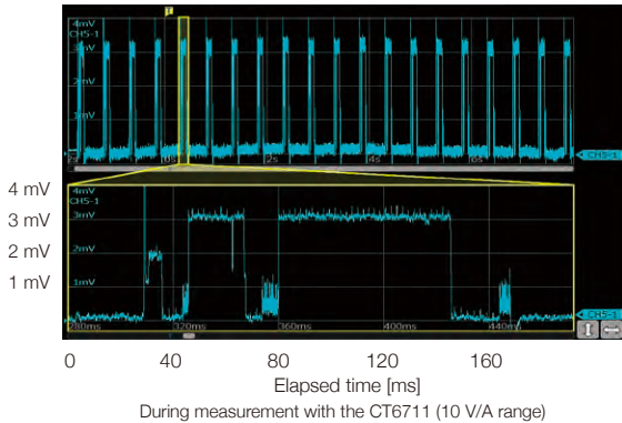
During measurement with the CT6711 (10 V/A range)
