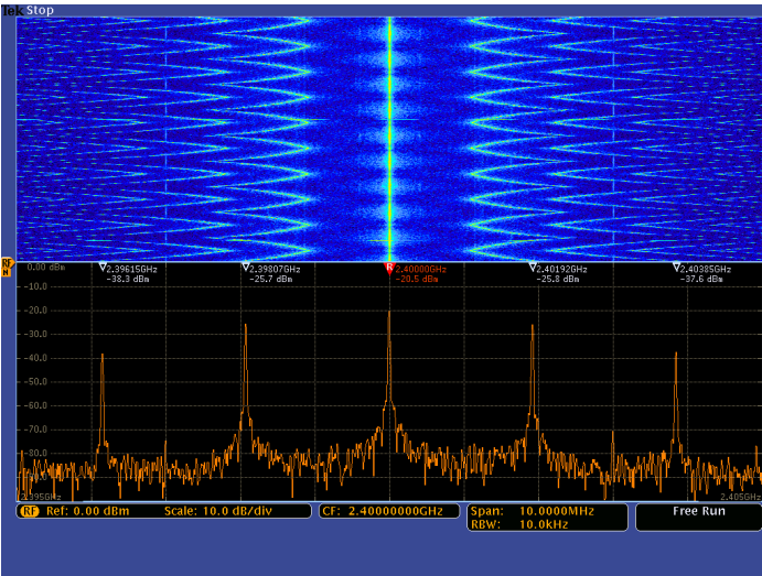
Spectrogram display illustrates slowly moving RF phenomena. As shown here, a signal that has multiple peaks is being monitored. As the peaks change in both frequency and amplitude over time, the changes are easily seen in the Spectrogram display.
