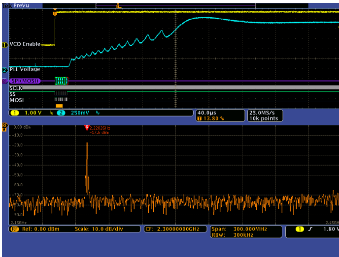
Figure 1 - Time and Frequency Domain view showing the turn-on of a PLL. Channel 1 (yellow) is probing a control signal that enables the VCO. Channel 2 (cyan) is probing the VCO tune voltage. The SPI bus which is programming the PLL with the desired frequency is probed with three digital channels and automatically decoded. Notice Spectrum Time is placed after the VCO was enabled and coincident with the command on the SPI bus telling the PLL the desired frequency of 2.400 GHz. Note that the RF is at 2.2202 GHz when the circuit turns on.
