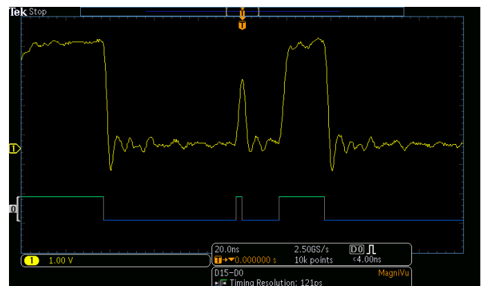
The MagniVu high-resolution record provides 121.2 ps timing resolution, enabling you to take critical timing measurements on your digital waveforms.
