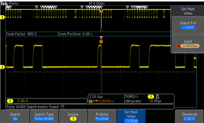
Search Step 1: You define what you would like to find. Automated measurement readouts provide repeatable, statistical views of waveform characteristics.
