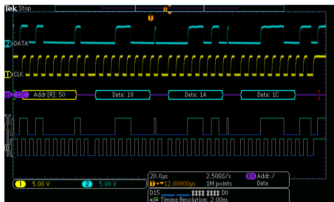
Triggering on a specific address and data packet going across an I2C bus. The yellow waveform is clock and the blue waveform is the data. A bus waveform provides decoded packet content including Start, Address, Read/Write, Data, and Stop.
