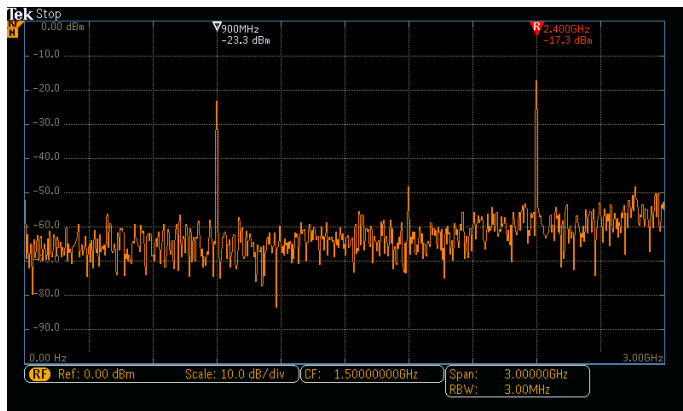
Spectral display of a bursted communication both into a device through Zigbee at 900 MHz and out of the device through Bluetooth at 2.4 GHz, captured with a single acquisition.
