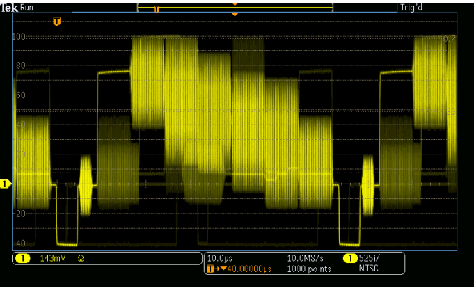
Viewing an NTSC video signal. Notice the intensity-graded view provided by the MDO3000's ability to represent time, amplitude, and distribution over time.
