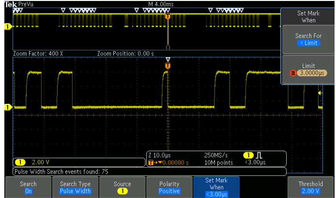
Search Step 1: You define what you would like to find. Automated measurement readouts provide repeatable, statistical views of waveform characteristics.
