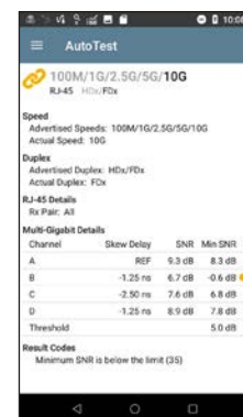
Cabling SNR measurement validates Multi-Gig links
