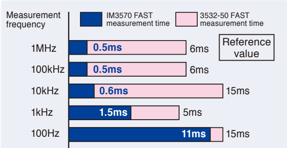
Comparison of measurement time of IM3570 and 3532-50
