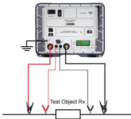
Figure 3. Connecting GGT to test object
