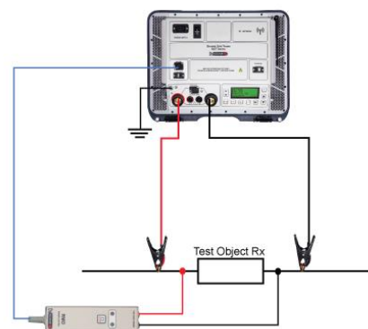
Figure 5. Connecting remote control unit to GGT
