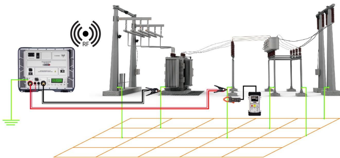
Figure 1. GGT connection for ground grid test
