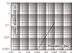
Measurable conductor diameter \Phi 20 mm (0.79 in)
