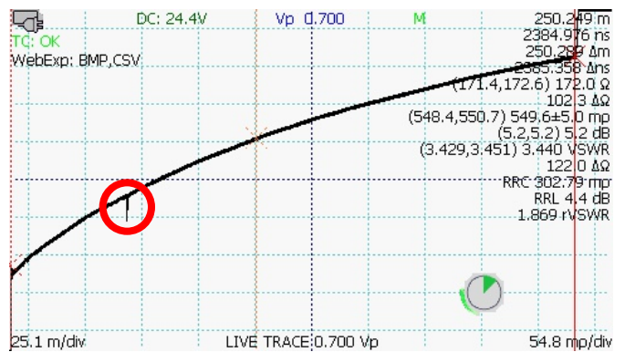
Figure 2: Subpixel fault easily identified on a long cable.
