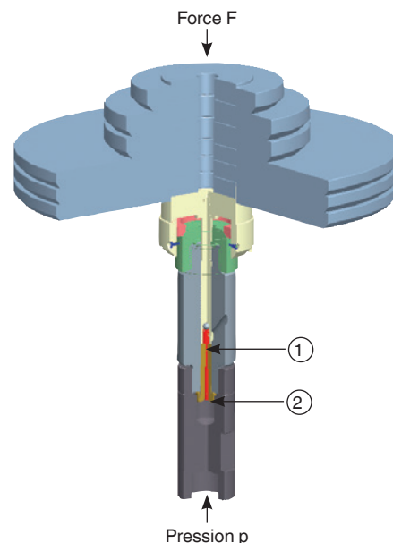
Ensemble piston-cylindre double gamme, 2.600 bar (40.000 lb/in 2 )
