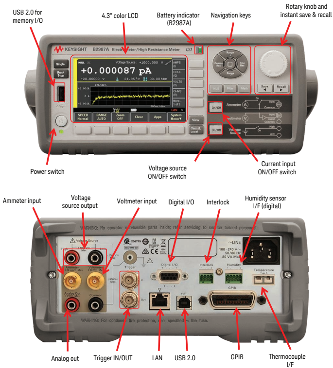
B2985A, B2987A Electrometer/High Resistance Meter
