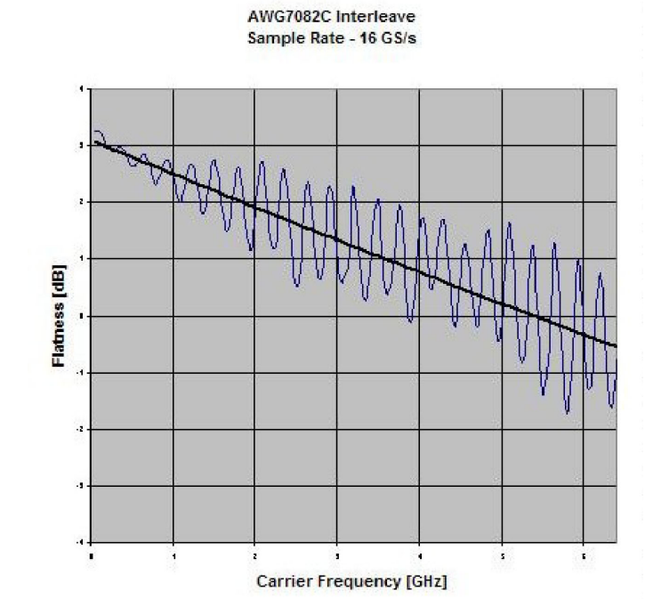
AWG7082C Interleave Flatness (typical).
