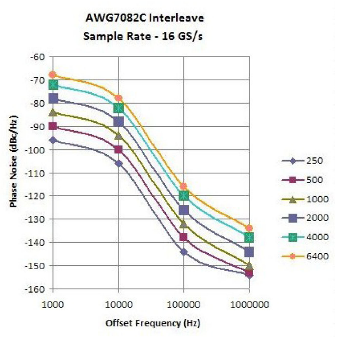
AWG7082C Interleave Phase Noise (typical).
