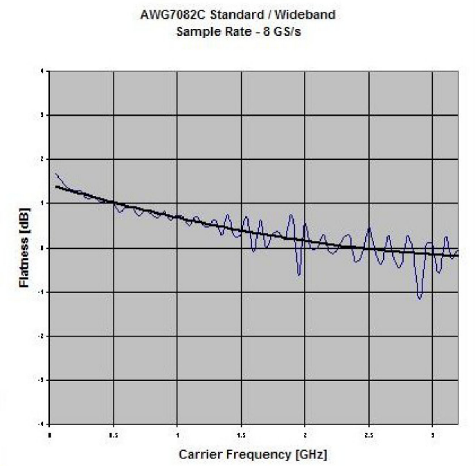
AWG7082C Standard/Wideband Flatness (typical).
