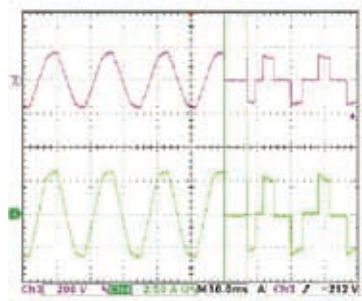
Figure 7: Transfer time for Off-Line UPS
