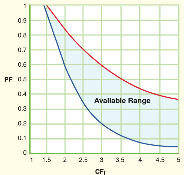
Figure 1: Crest Factor vs. Power Factor control Range
