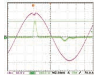
Figure 6: Inrush Current Mode
