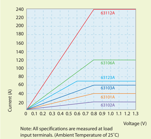
Low Voltage Characteristics (Typical) Model 63101A/63102A/63103A/63106A/63112A/63123A
