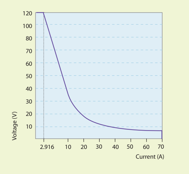
Model 63123A Input Characteristics
