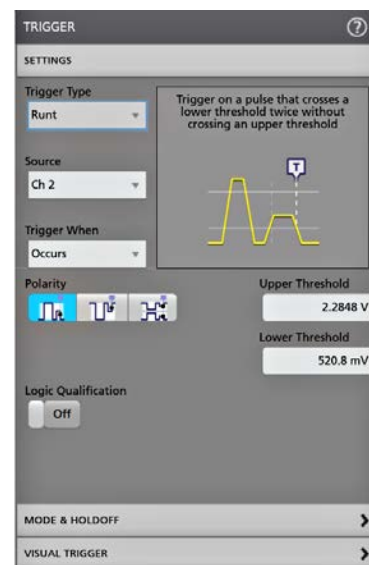
Figure 8: Configuration menus are accessed by simply double-tapping on the item of interest on the display. In this case, the Trigger badge was double-tapped to open the Trigger configuration menu.
