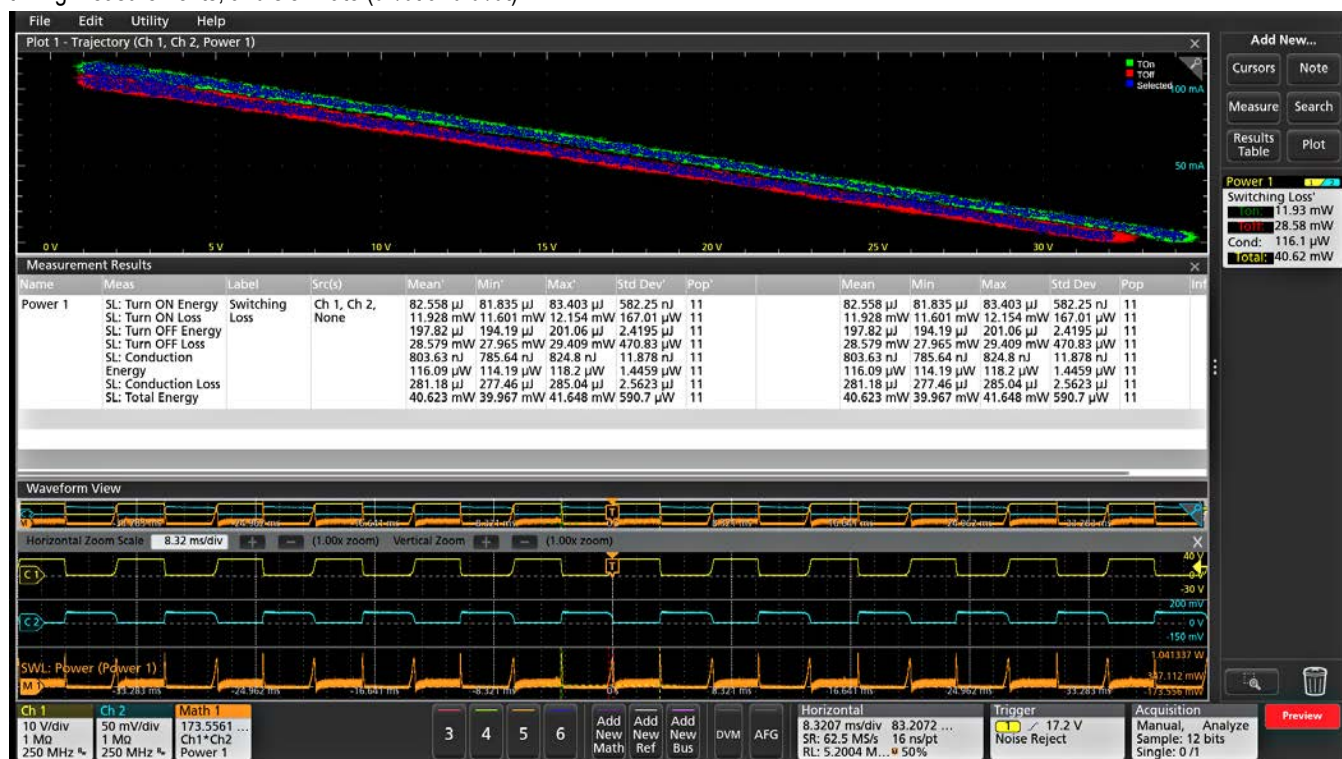
Figure 27: The Power Analysis measurements display a variety of waveforms and plots.
