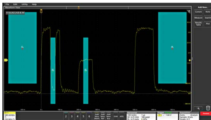
Figure 15: Visual Trigger areas isolate an event of interest, saving time by only capturing the events you want to see.
