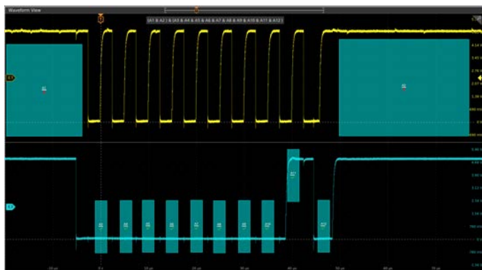
Figure 16: Multiple channel triggering. Visual Trigger areas can be associated with events spanning multiple channels, such as triggering on a specific burst-width on channel 1 and a specified bit pattern on channel 2.
