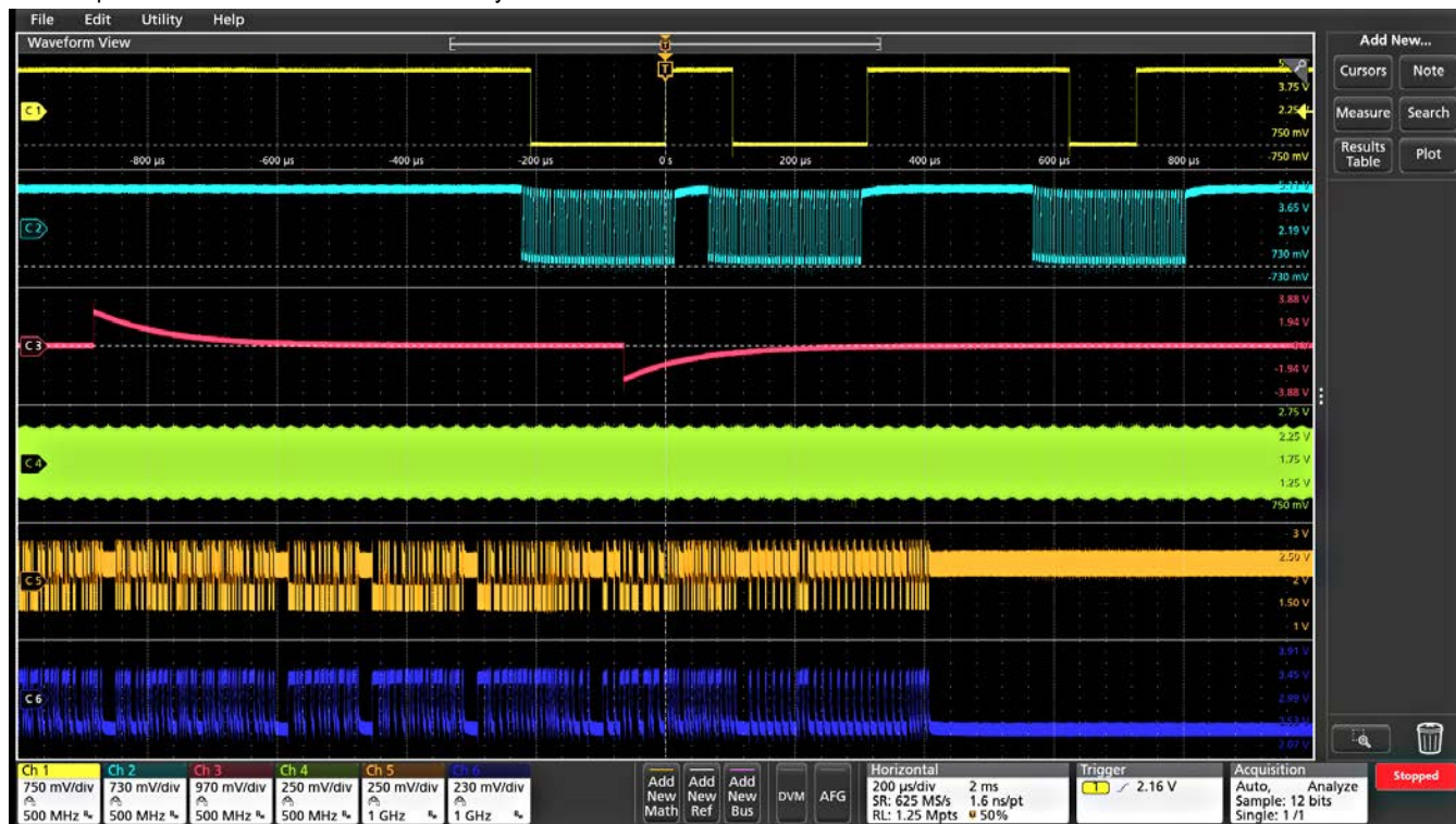
Figure 6: Stacked display mode enables easy visibility of all waveforms while maintaining maximum ADC resolution on each input for the most accurate measurements.
