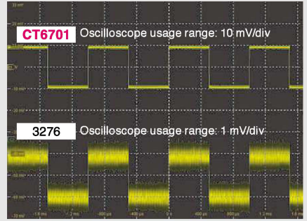
Input: 20 mAp-p, 1 kHz, square wave Oscilloscope: Bandwidth 2 GHz, 10 mV/div
