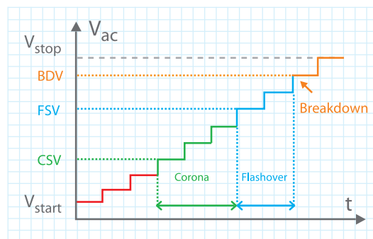
Figure 4: Discharge Level Analysis (DLA)
