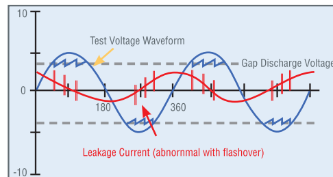
Figure 2: Flashover Waveform
