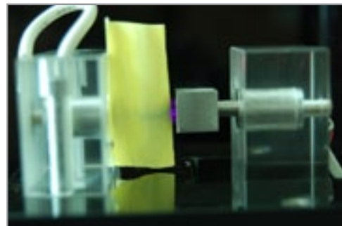
Figure 1: Corona Discharge
